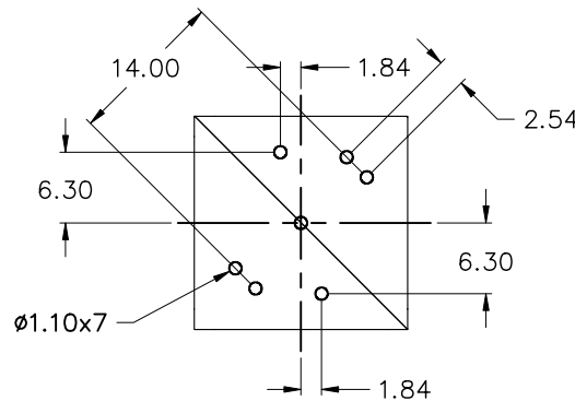
P.C. MOUNTING
