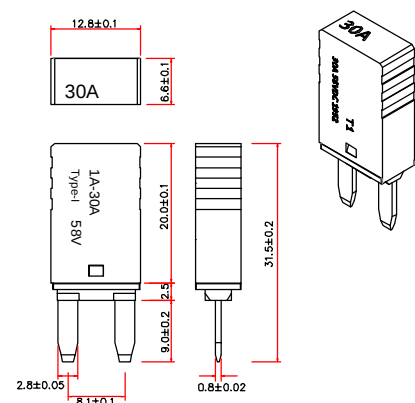
Auto Reset (Type I)
