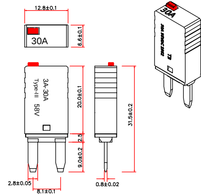
Manual Reset (Type III)
