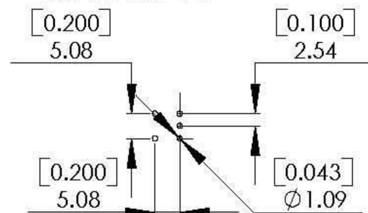
P.C. MOUNTING
