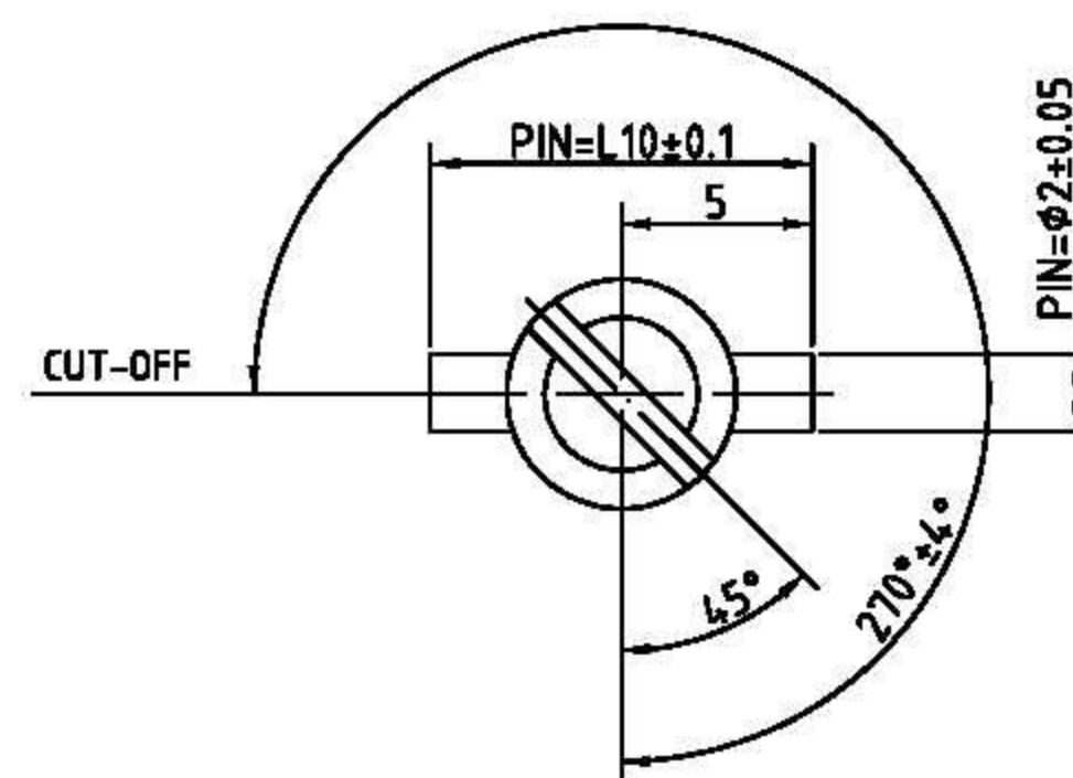
#SHAFT OUTSIDE DIMENSION
