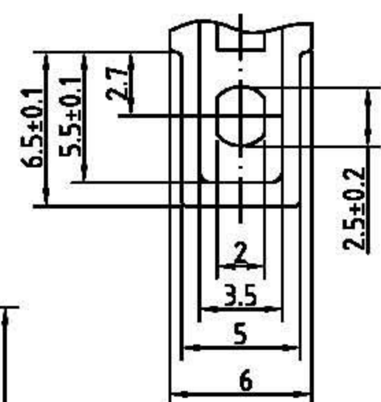
TERMINAL #187 OUTSIDE DIMENSION
