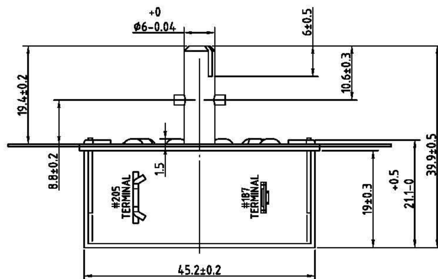
TERMINAL #187 OUTSIDE DIMENSION
