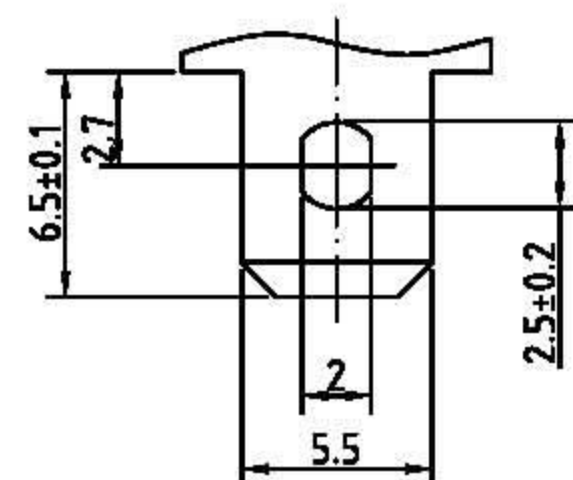
TERMINAL #205 OUTSIDE DIMENSION
